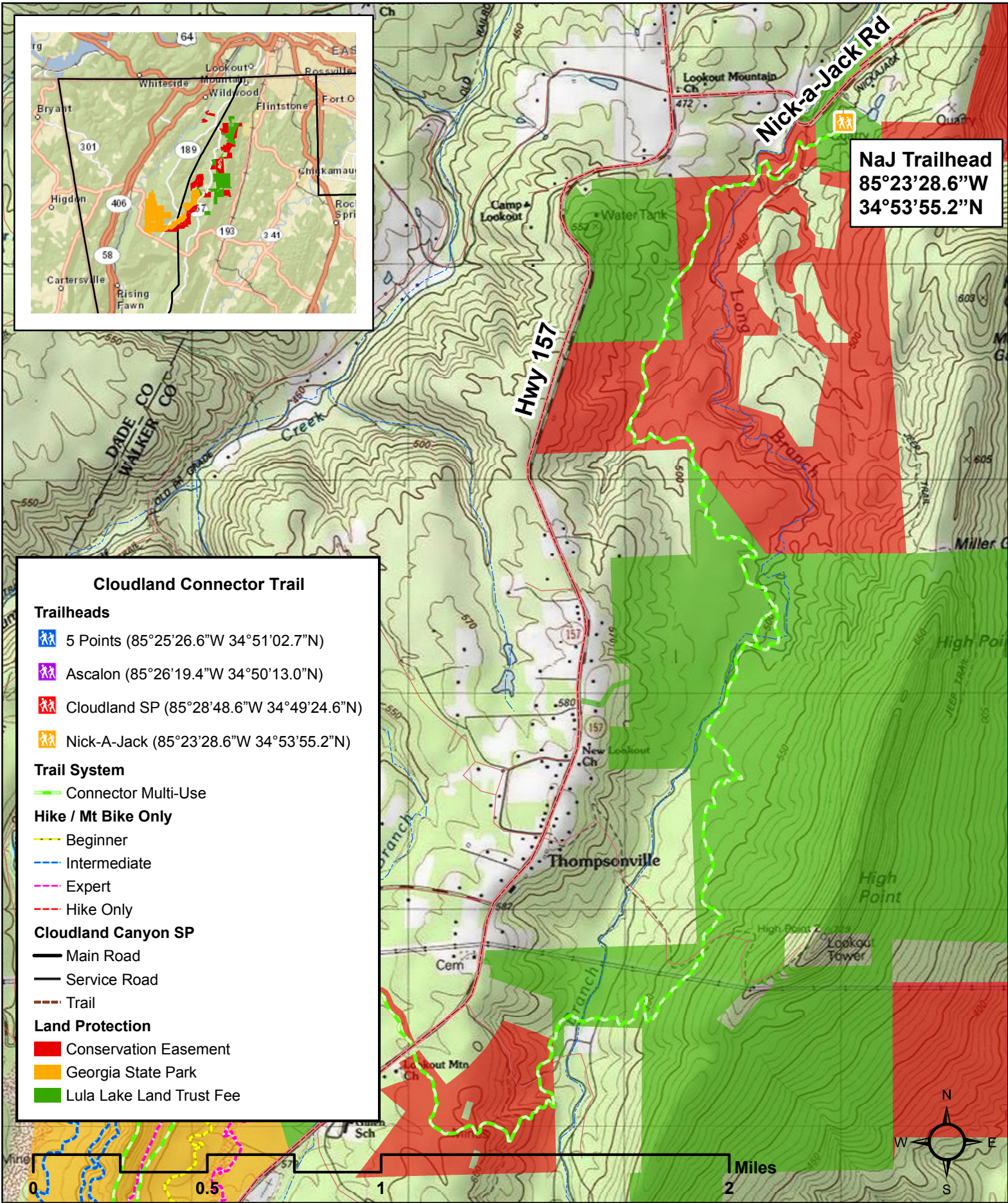
Clouland Connector Trail Clouland Canyon State Park Phase I Trail Layout Map
